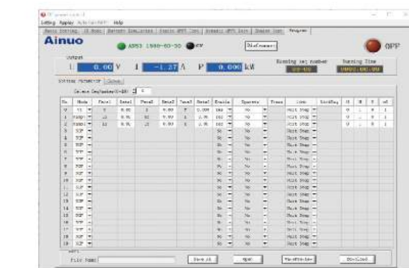
EN50530 Dynamic Simulation
